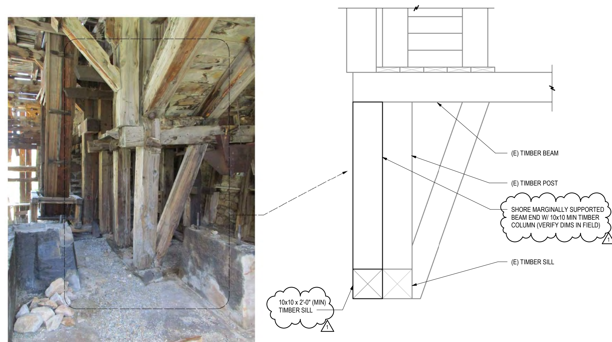
1 SECTION S511 1/2" = 1'-0"
